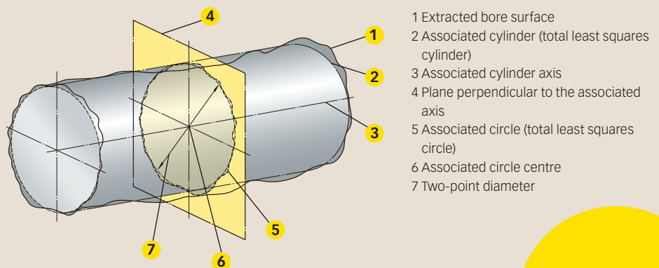
Fig. 7: Association for two-point size on a cylinder.
